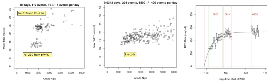
Fig. 7. (left) Identified RPR low background events in DRIFT IId. (middle) Low energy ( > 40 keV) calibration sulphur recoils from a neutron exposure (gamma rejection is > 10^8 ). (right) Rise in ^{210}\text{Po} RPR events with time following new gas fill fitted to expectation of RPR hypothesis. From Ref. 39.
